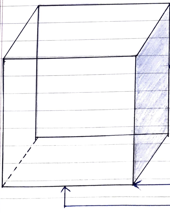
Cube
