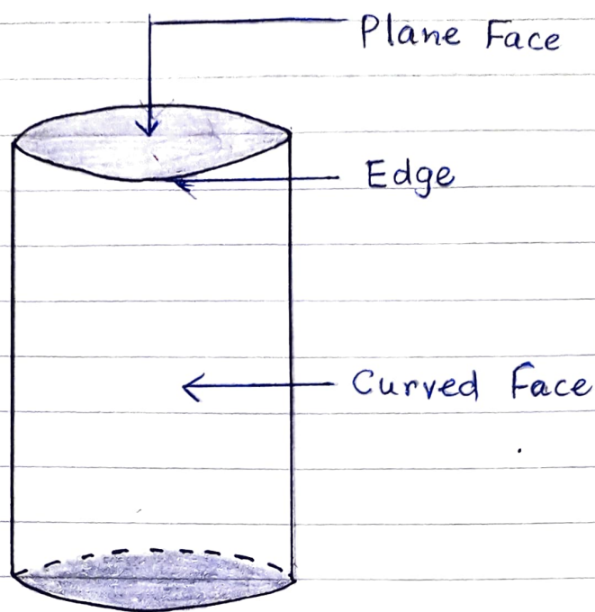
Cylinder
